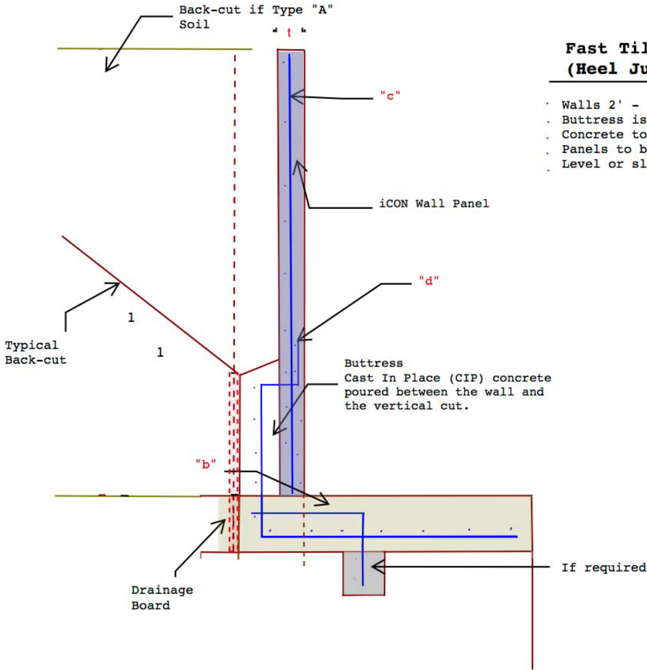
Sample- Retaining Wall schedule (2000psf) - Cut Soil
